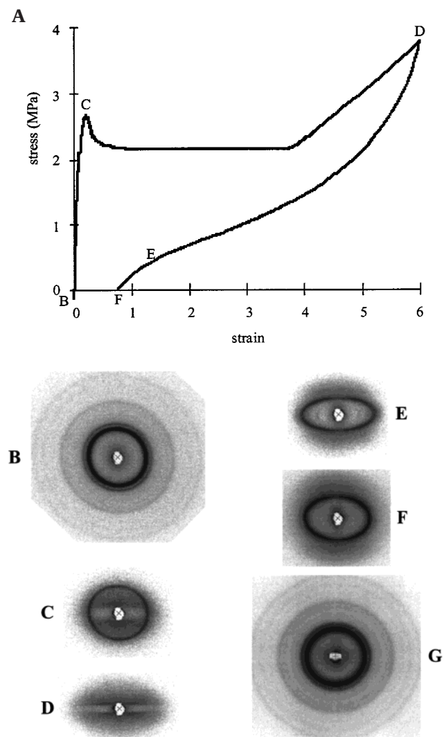
Figure 4. (A) Stress-strain curve of an isotropic, polygranular 34% S SIS DG (top), with accompanying SAXS patterns. (B) Pattern at start before deformation. (C) Pattern at yield, ~20% strain. (D) Pattern at 600% strain. (E) Pattern unloaded to ~130% strain. (F) Pattern fully unloaded, with ~70% residual strain. (G) Pattern upon annealing at 120 °C for 2 weeks.
